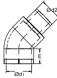
PP-R 45° KUYRUKLU DİRSEK PN 25
